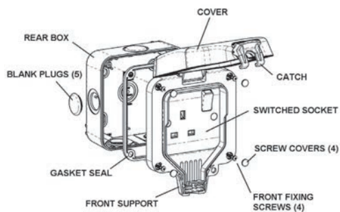
1 GANG SWITCHED SOCKET – EXPLODED VIEW
